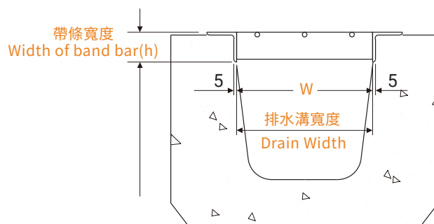
GU排水格柵 GU Type Drainage Grating
