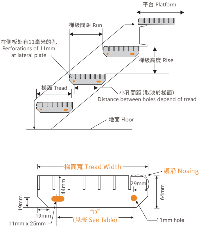
樓梯踏板典型細節 STAIR TREADS TYPICAL DETAIL
